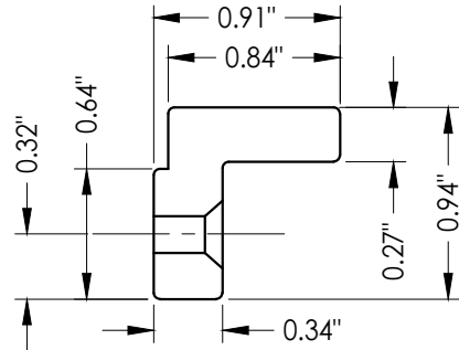
24 TILT LATCH BLOCK
