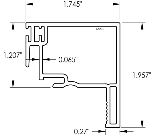
7 LOCK RAIL
