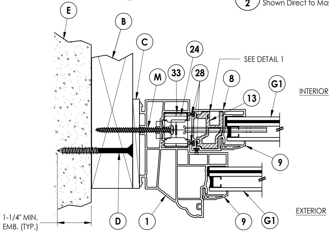
1 HORIZONTAL CROSS SECTION 2X Buck Construction
