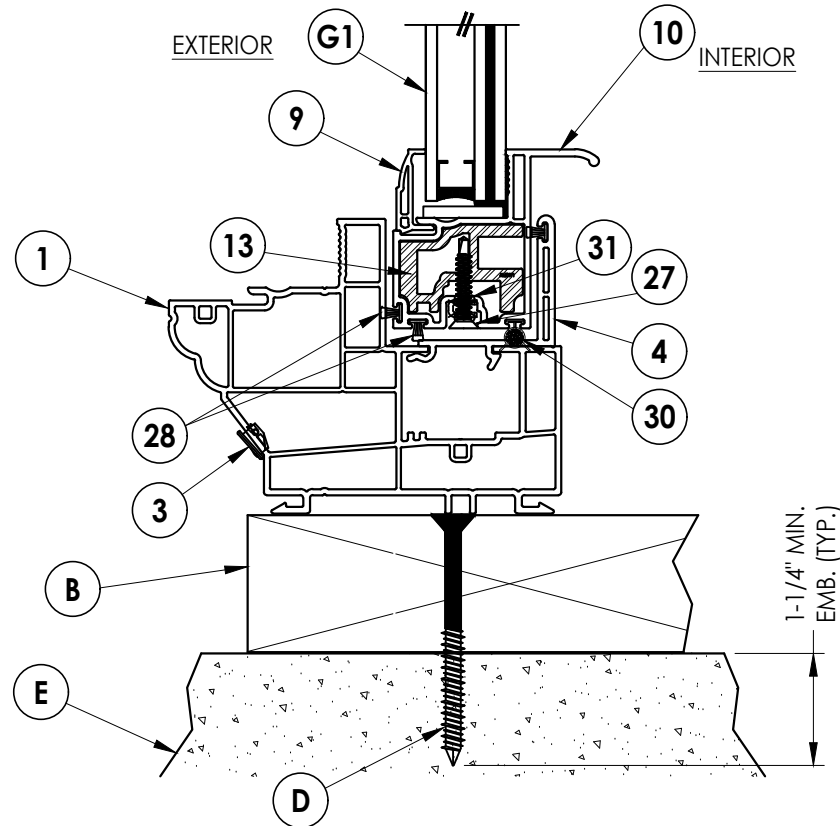
4 4 VERTICAL CROSS SECTION 2X Buck Construction
