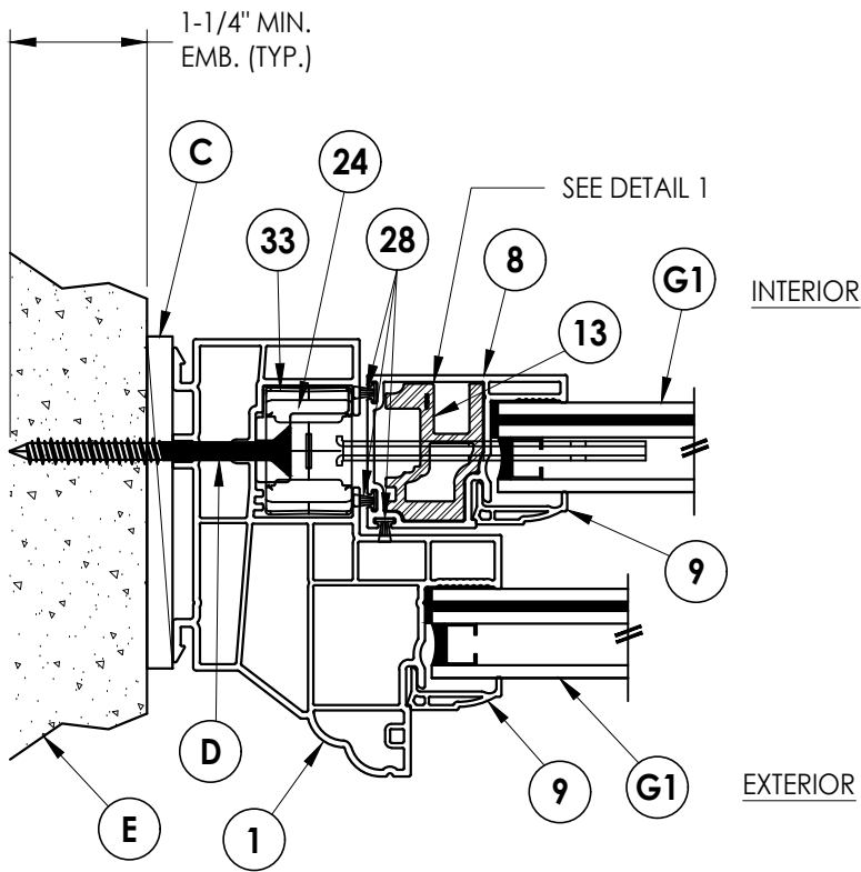
2 HORIZONTAL CROSS SECTION Shown Direct to Masonry
