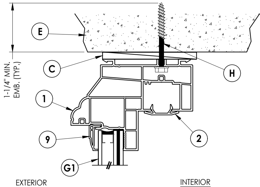
2 4 VERTICAL CROSS SECTION Shown Direct to Masonry
