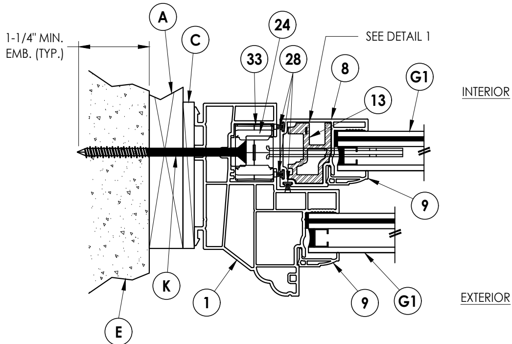
3 HORIZONTAL CROSS SECTION Shown w/ 1X Buck
