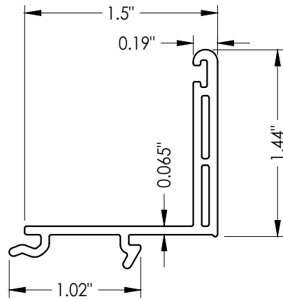
4 SILL ADAPTER
