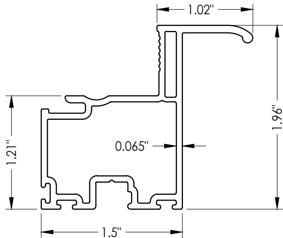
10 LIFT RAIL
