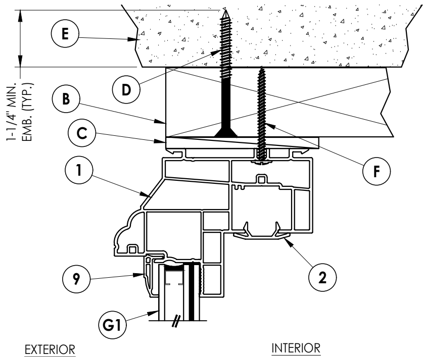
1 4 VERTICAL CROSS SECTION 2X Buck Construction
