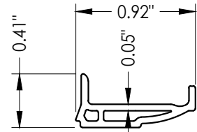
9 GLAZING BEAD
