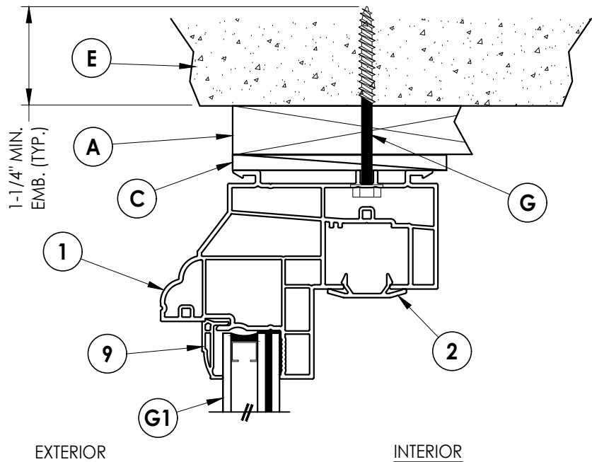
3 4 VERTICAL CROSS SECTION Shown w/ 1X Buck
