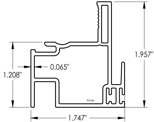
6 KEEPER RAIL
