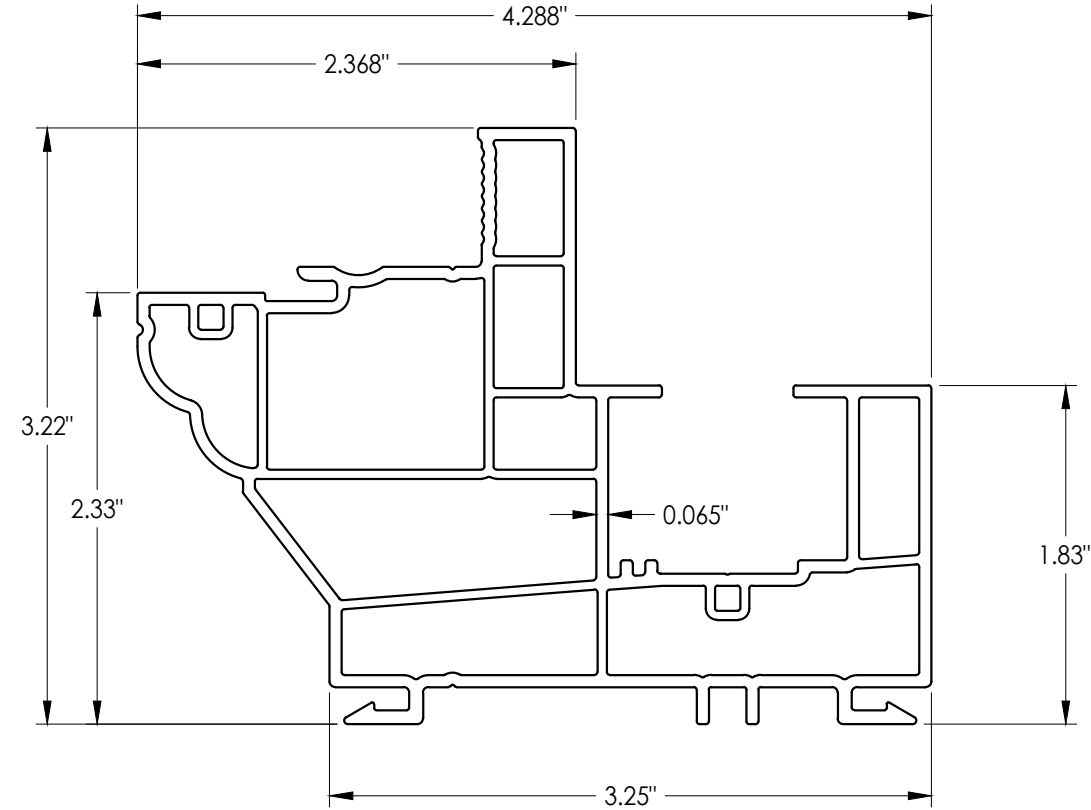
1 FRAME
